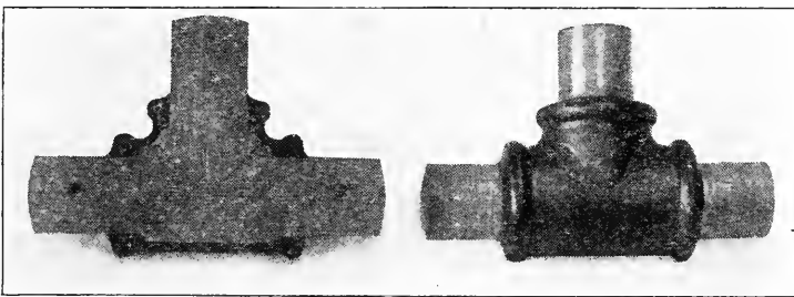
FIG. 568. MITERED MEMBERS OF PATTERN FOR TEE-PIPE FITTING.
